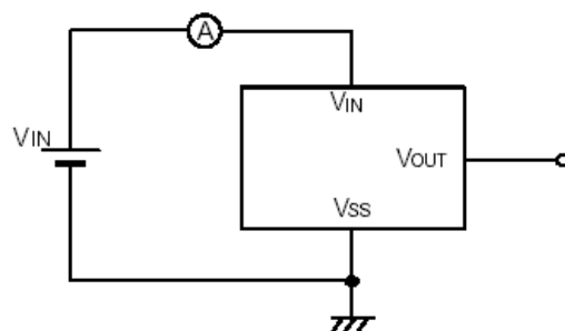
Circuit 4
