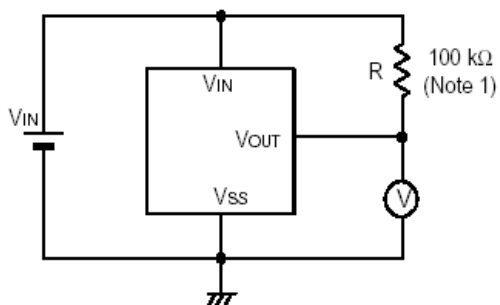
Circuit 3
