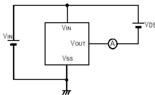
Circuit 4
